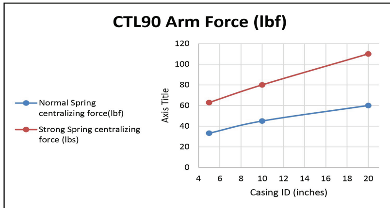
Centralizing Force Chart for CTL90 Centralizers
